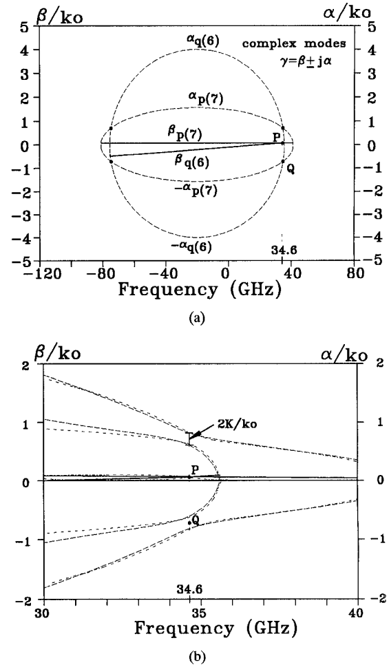
Fig. 7. Mode-coupling between two complex modes. The solid and dashed lines represent the normalized propagation constant and attenuation constant, respectively. The dashed-dotted lines represent the corresponding coupled-mode solutions \gamma_1 and \gamma_2 . (a) Two hypothetical modes \gamma_p and \gamma_q obtained directly from Fig. 3 using the procedure described in Section VI-B, where the corresponding straight lines for obtaining the two ellipses are: F_6B_6 : a/ko = 0.0770 , b/ko = 1.34 , c/ko = -0.067 , d/ko = -1.54 , K/ko = 4.0 ; F_7B_7 : a/ko = 0.0256 , b/ko = 0.31 , c/ko = 0.0256 , d/ko = -0.712 , K/ko = 1.57 . (b) Comparison of the mode spectrum obtained by SDA and mode-coupling (5) and (6) using \gamma_p and \gamma_q , i.e. two ellipses, obtained in (a). K/ko = 0.1 .
