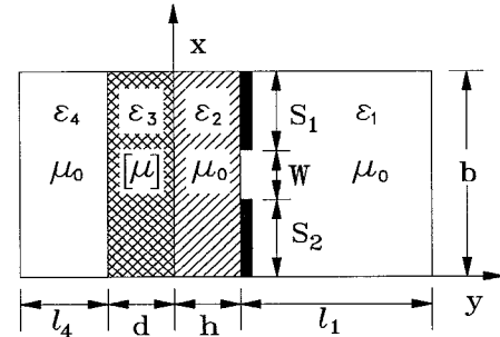
Fig. 2. Cross-sectional geometry of a unilateral finline integrated on the stratified layers containing a ferrite substrate magnetized in x -direction. The structural and material parameters are: l_1 = 3.556 mm, d = h = 1 mm, l_4 = 1.556 mm, b = 3.556 mm, s_1 = s_2 = 1.628 mm, w = 0.3 mm, \epsilon_1 = \epsilon_4 = 1 , \epsilon_2 = \epsilon_3 = 12.5 , 4\pi Ms = 4900 G, and H_0 = 500 Oe.
